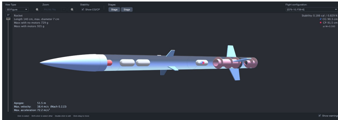
*OpenRocket Model with Stability and Approximate Dimensions
